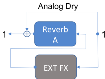
Toggle Switch = Reverb A
